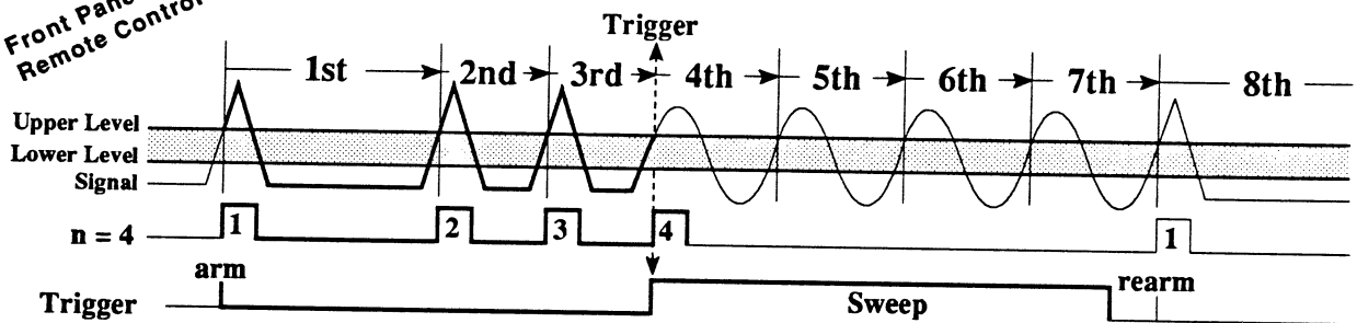
Figure 1 - n Event-Interval - The counter is set to four ( n = 4 ). The counter counts only qualified positive slope events and triggers the sweep when it reaches a count of four (4). This example illustrates positive slope triggering.
