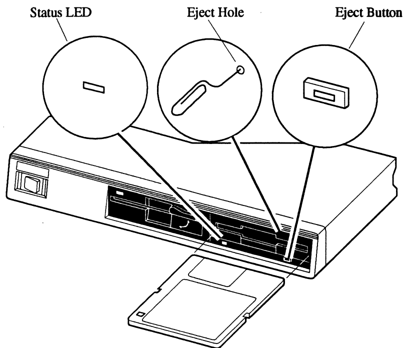
Figure 1 - Pro Disk Optical cartridge drive
