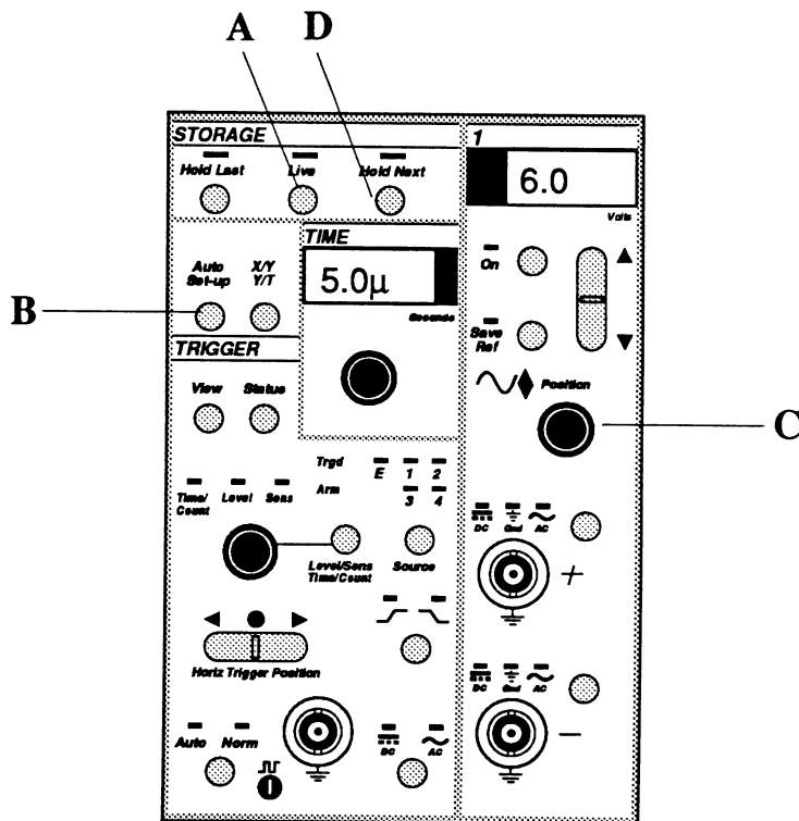
Figure 1 - Using the Compensation Point as the signal source for channel 1.
