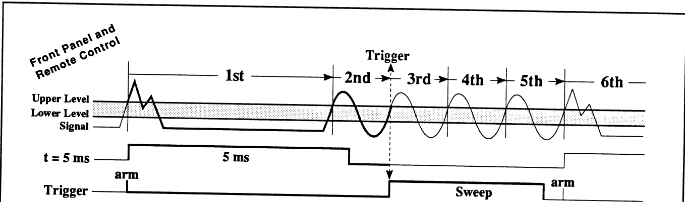
Figure 1 - Hold Off-Interval - The timer is set to 5 ms. The positive slope event in the 1st cycle starts the timer, thus holding off the positive slope event at the start of the 2nd cycle from triggering a sweep. The timer finishes timing out during the 2nd cycle which now allows the positive slope in the 3rd cycle to trigger a sweep. This example illustrates positive slope triggering.
