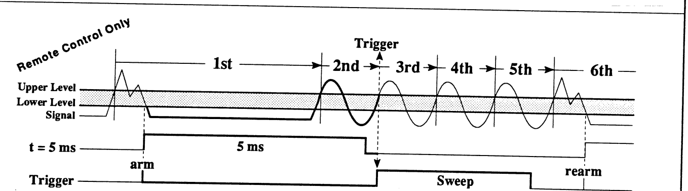
Figure 2 - Hold Off-Pulse Width - The timer is set to 5 ms. The negative slope event in the 1st cycle starts the timer, thus holding off the positive slope event at the start of the 2nd cycle from triggering a sweep. The timer finishes timing out during the 2nd cycle which now allows the positive slope at the start of the 3rd cycle to trigger a sweep. This example illustrates positive slope triggering.
