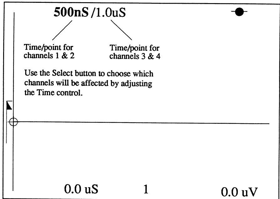
Figure 1 - The Time Per Point has been set to 500 nS for channels 1 and 2, and 1.0 \mu S for channels 3 and 4 in this example. Use the Select button to choose which pair of channels will be set when you adjust the Time control.
