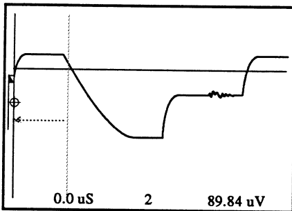
Figure 2 - The Horizontal Cursor moves to the trigger time ( t=0 ) origin when the Left and Right Cursor buttons are pressed simultaneously.
