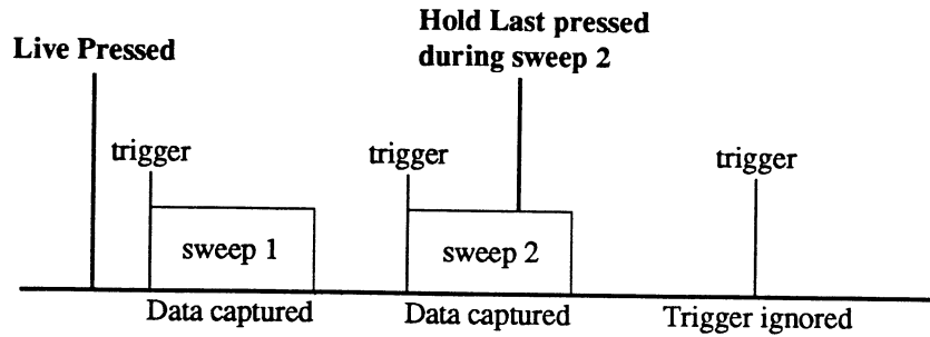
Figure 1 - Hold Last was pressed during the second sweep. The second sweep is allowed to complete and the captured data remains displayed on the screen.
