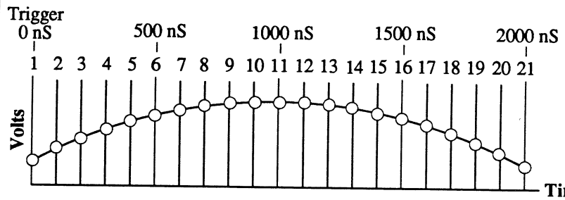
Figure 1 - Analog input signal superimposed with the 100 nS sampling rate. The Sweep Length setting will determine which of the samples are digitized.
