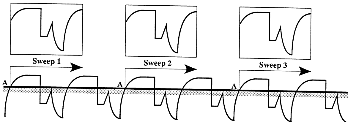
Figure 4 - Solution #2: Eliminating Feature B by raising the trigger Level above Feature B.
