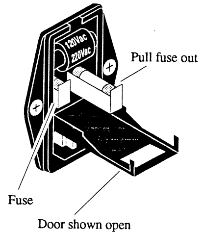
Figure 2 - Replacing the Fuses
