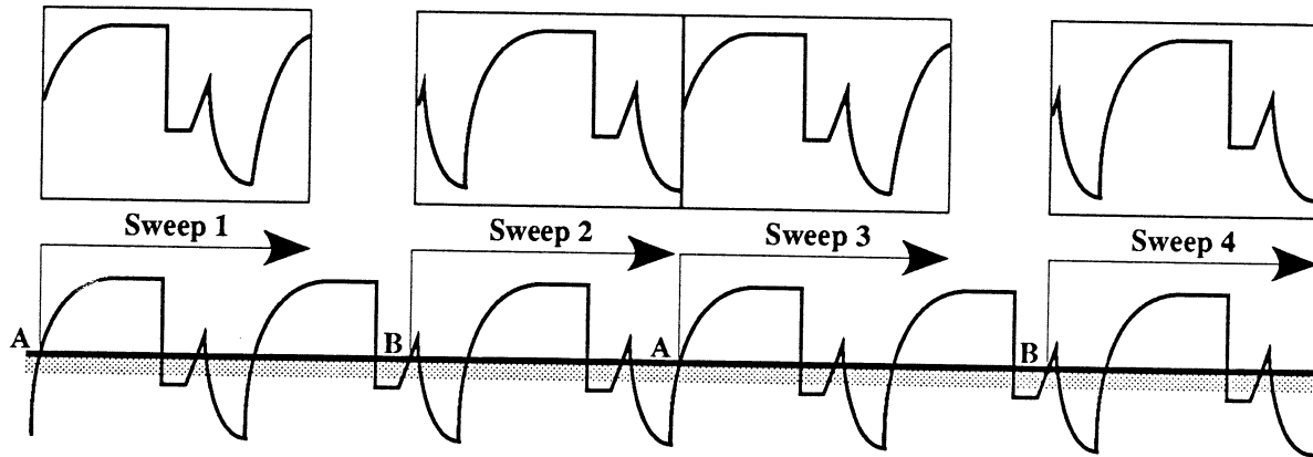
Figure 2: Example of an unstable display caused by nonperiodic triggering off of Features A and B.
