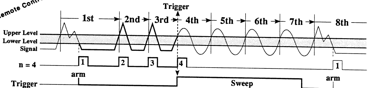
Figure 2 - n Event-Pulse Width - The counter is set to four ( n = 4 ). The counter counts the first qualified negative slope event and then only qualified positive slope events thereafter. A sweep is triggered when the counter reaches a count of four (4). This example illustrates positive slope triggering.
