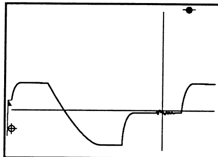
Figure 4 - Autocenter was turned on and the crosshair was positioned over the area of interest on the unexpanded waveform.
