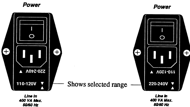
Voltage Selector set for 110-120V Voltage Selector set for 220-240V
