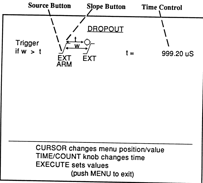
Figure 1 - Positive slope triggering is selected and the trigger source is set for the External input BNC. A sweep is triggered if the 999.2 \mu S timer times out before it is reset by a qualified event.
