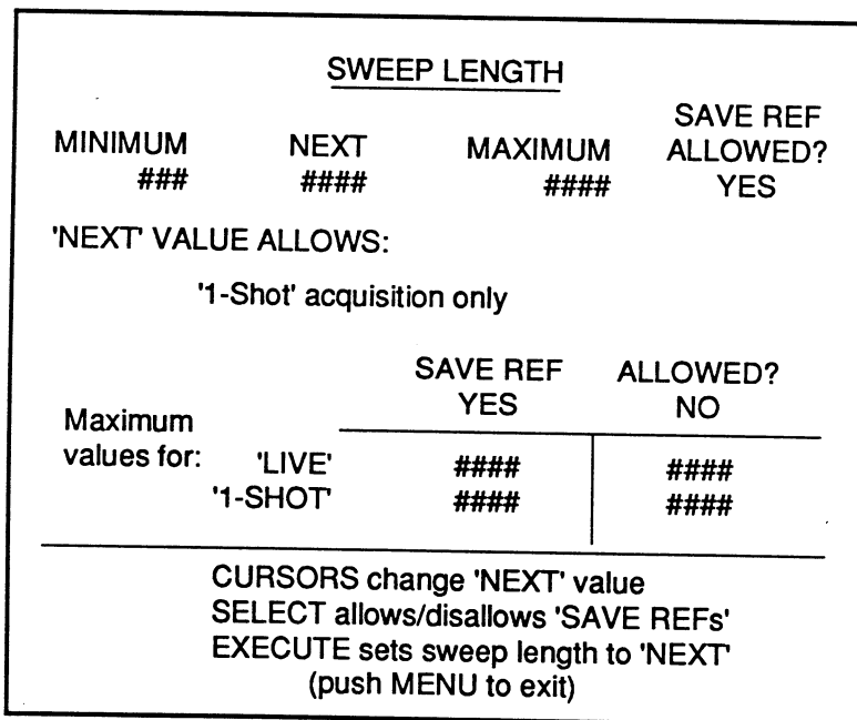
Figure 2 - Sweep Length parameter screen when the 'MAXIMUM' sweep length value is entered in the 'NEXT' field.
