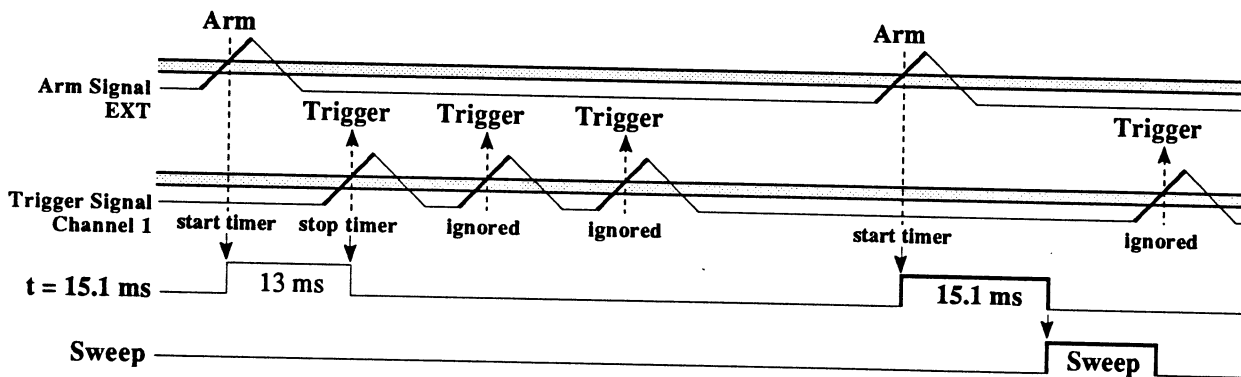
Figure 2 - ADV Triggering - Drop Out Answering with a YES for the "Re-arm required if trigger occurs during t?" parameter, the instrument measures Arm-to-Trigger time. If a valid Trigger occurs while the timer is timing, the timer stops and another valid Arm signal is required to start the timer again at t=0 . If the timer times out, a sweep is triggered. The timer is re-armed by the next valid Arm signal after the sweep ends and then the next valid Trigger signal starts the timer.
