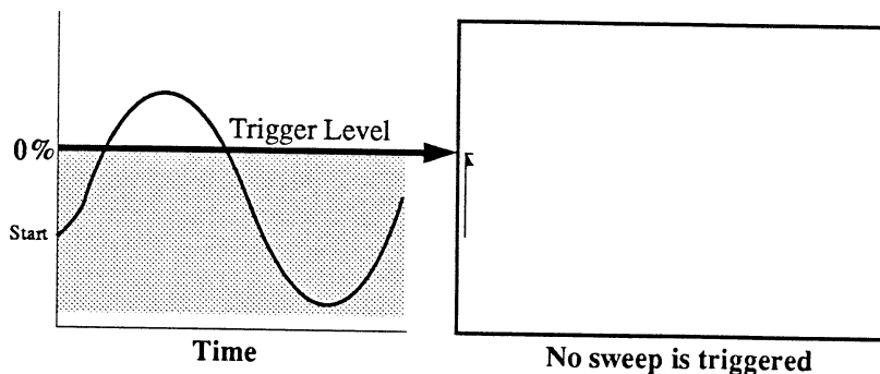
Figure 2 - This signal failed to trigger a sweep because it did not begin its initial positive voltage transition outside the Sensitivity window.
