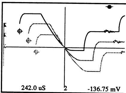
Figure 5 - The waveform passes through the crosshair locked at screen center when Horizontal Expansion, Vertical Expansion and Autocenter are all turned on and the Left or Right Cursor button is pressed.
