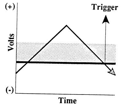
Figure 5 - The signal qualifies as a negative trigger.
