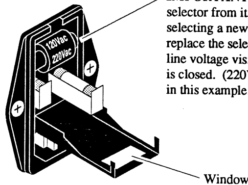
Figure 3 - The Voltage Selector
