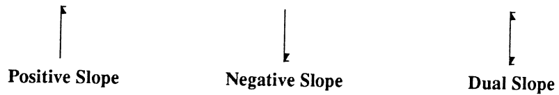
Figure 1 - Trigger Slope Markers appear when View Mode is turned on.
