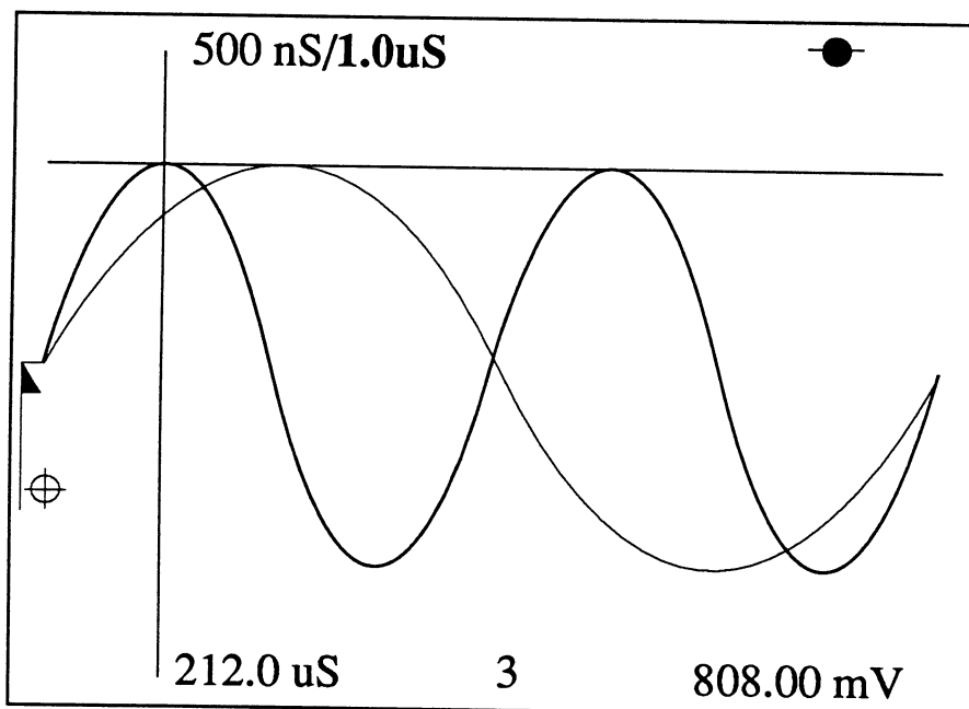
Figure 2 - Two identical signals were input to channels 1 and 3 with the Time Per Point settings shown. Channel 1 captured one full cycle with its Time Per Point setting of 500 nS and channel 3 captured two full cycles with its Time Per Point setting of 1.0 μS.
