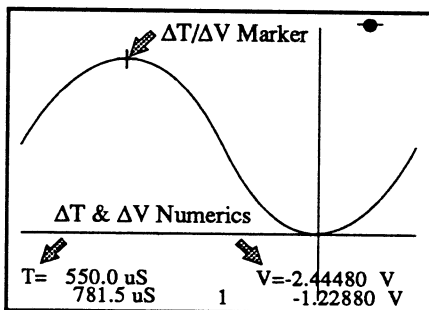
Figure 1 - The \Delta T/\Delta V Marker, Time Numerics and Voltage Numerics.
