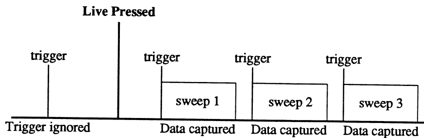
Figure 1 - The Live button was pressed, thus arming the instrument to start a sweep each time a valid trigger is received.
