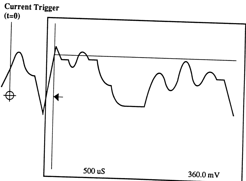
Figure 4 - After triggering a new sweep, the display now contains data that was captured 500 \mu S after the trigger occurred. Note that the time numerics now reads 500.0 \mu S.
