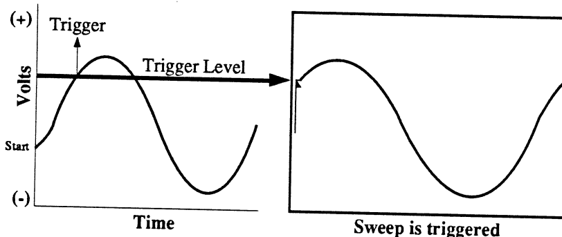
Figure 3 - The trigger Level was lowered, allowing the signal to qualify as a trigger.
