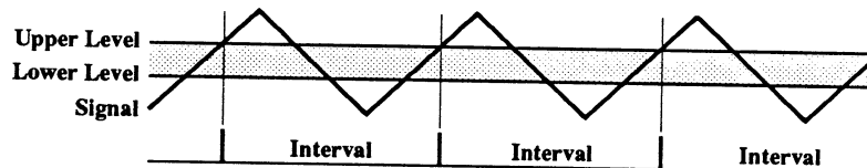
Figure 3 - When Positive Slope triggering is used, the Interval is the time span between two qualified rising edges of the selected signal.
