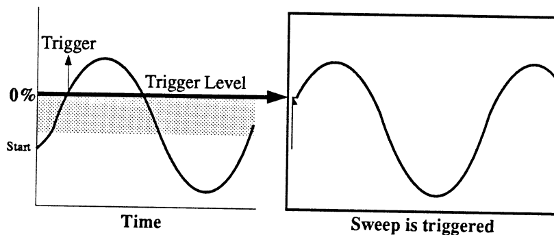
Figure 3 - The Sensitivity window was reduced. The signal qualified as a valid trigger because it started its positive voltage transition outside the Sensitivity window before it crossed the Trigger Level.
