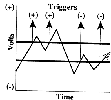
Figure 6 - The signal qualified as dual slope triggers at the points shown. Dual Slope triggering ignores the Sensitivity window. Only the Source, Slope and Level requirements have to be met.
