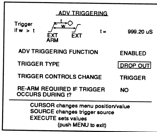
Figure 2 - Drop Out triggering is selected. Note that you can select to restart the timer. See the 'Drop out triggering selected' description above.
