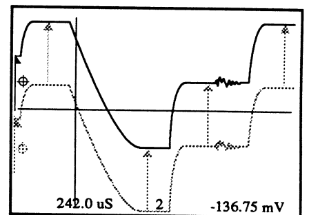
Figure 5 - The display screen "moves down" (the waveform appears to move up) when Vertical Expansion is turned on and the Down Cursor button is pressed.
