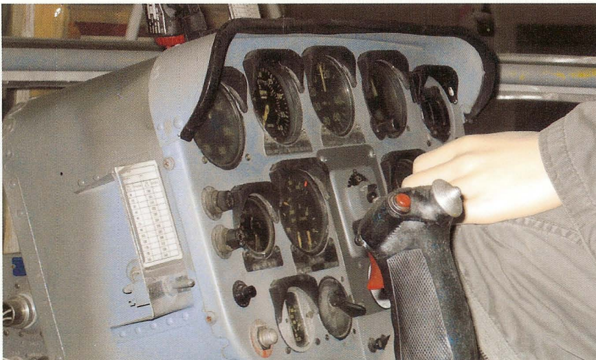
The simple instrument panel of the OH-13G was ideal for primary flight training. It was not so complex as to confuse the student.
