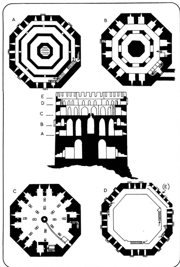
The Kizil Kule (Red Tower) at Alanya in southern Turkey was designed by a Syrian architect in 1224 for the Saljuq Sultan of Rum. It forms the focus of a defensive system for a major naval base.
