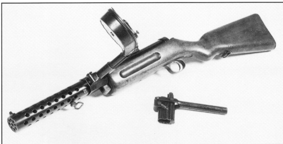
The MP18 was one of the first sub-machine guns to be used in action. Note the 32-round 'snail' magazine, developed for the Artillery Model Luger, and its loading tool. The magazine affects the balance of the MP18, canting the weapon sharply to the left even when empty. (Pattern Room Collection)
